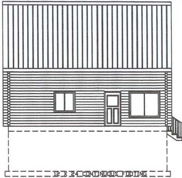
REAR ELEVATION
