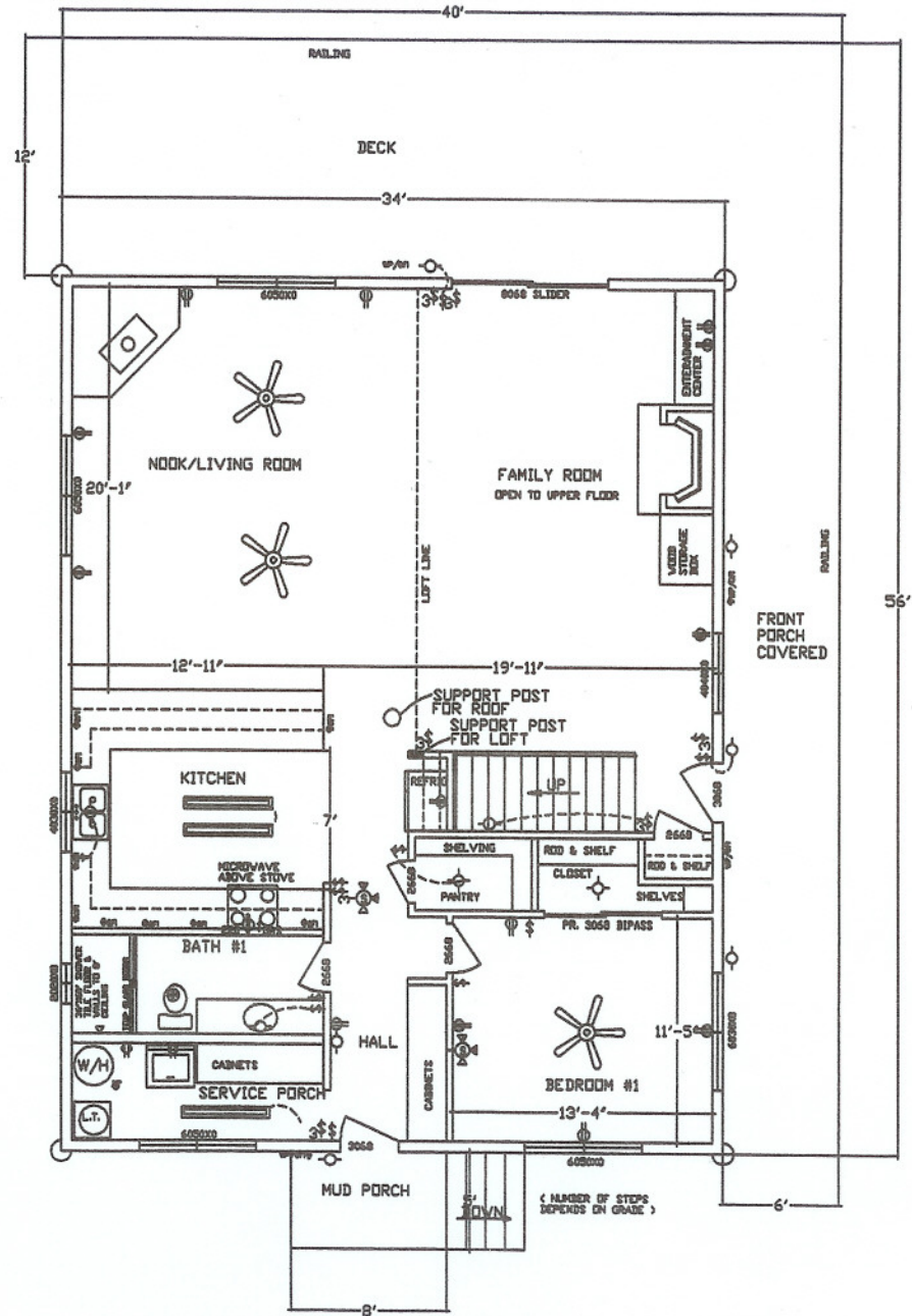
MAIN FLOOR PLAN 1496 SQ. FT.
