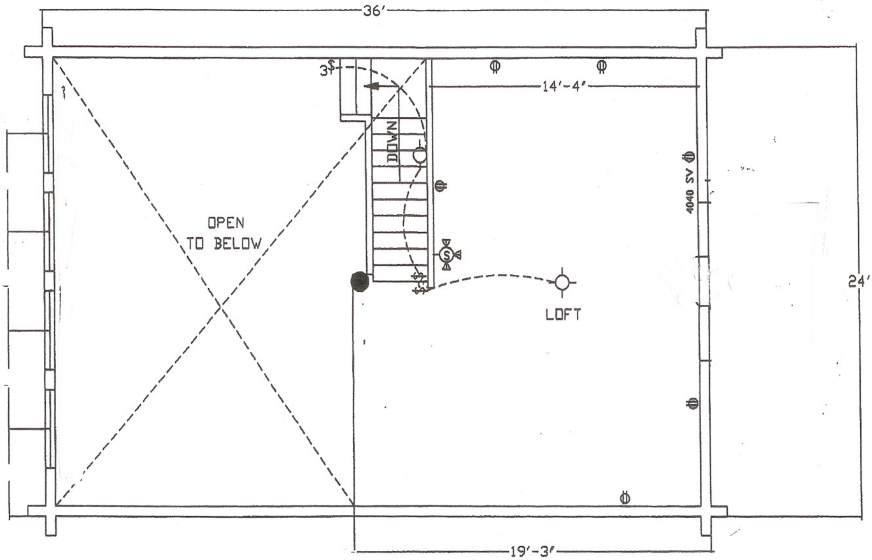
LOFT FLOOR PLAN 416 SQ. FT.
