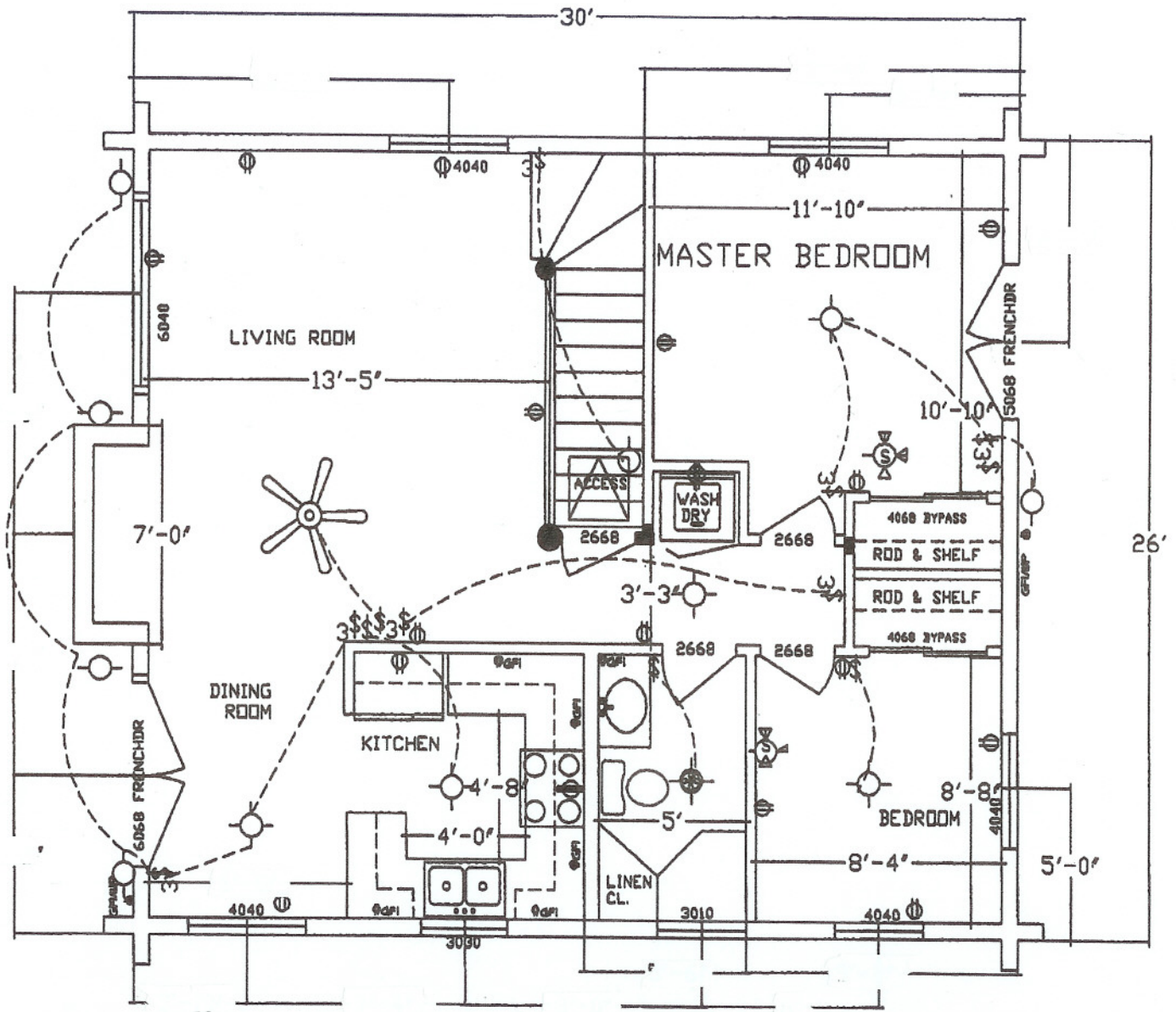
MAIN FLOOR PLAN 798 SQ. FT.
